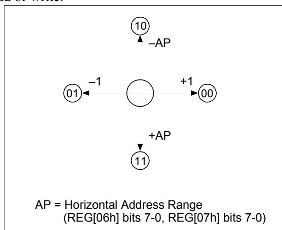
Figure 10-8 Cursor Direction
