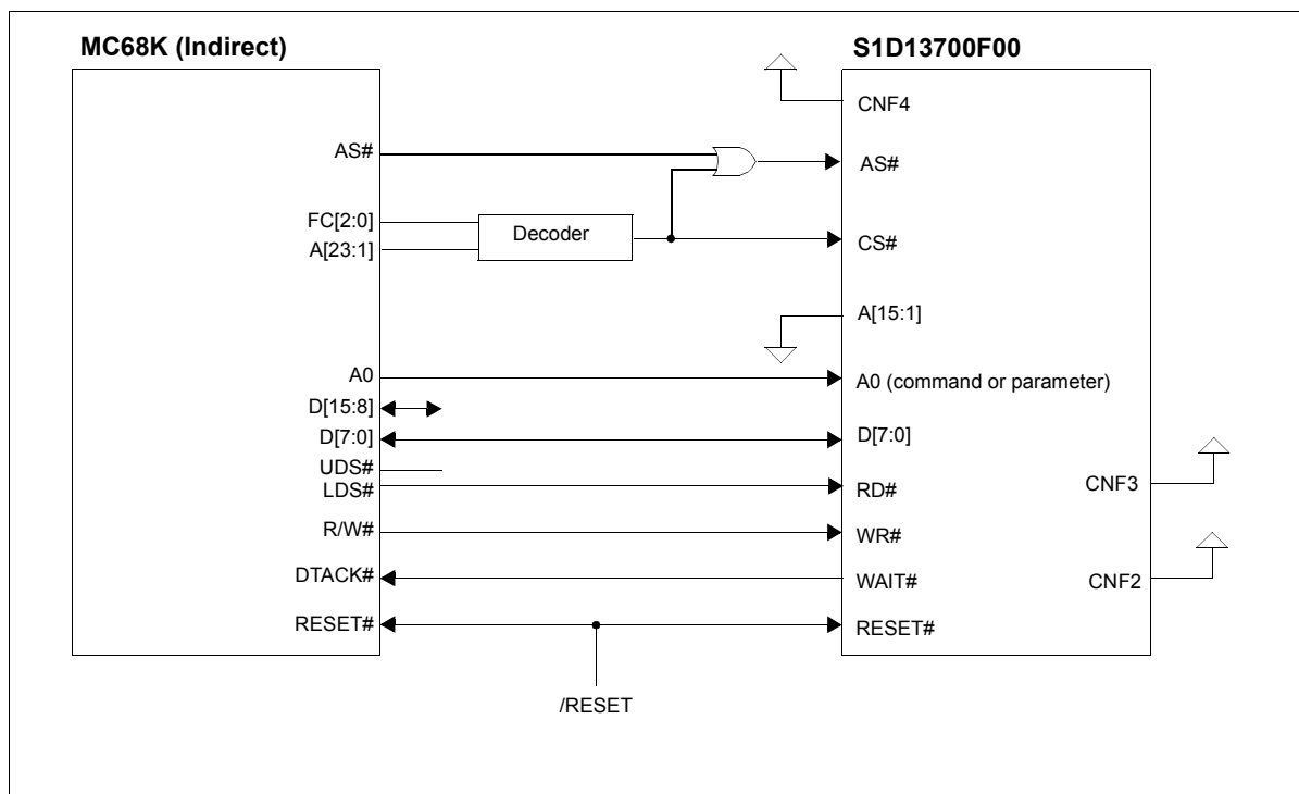
Figure 3-3 Indirect MC68K to S1D13700F00 Interface Example
