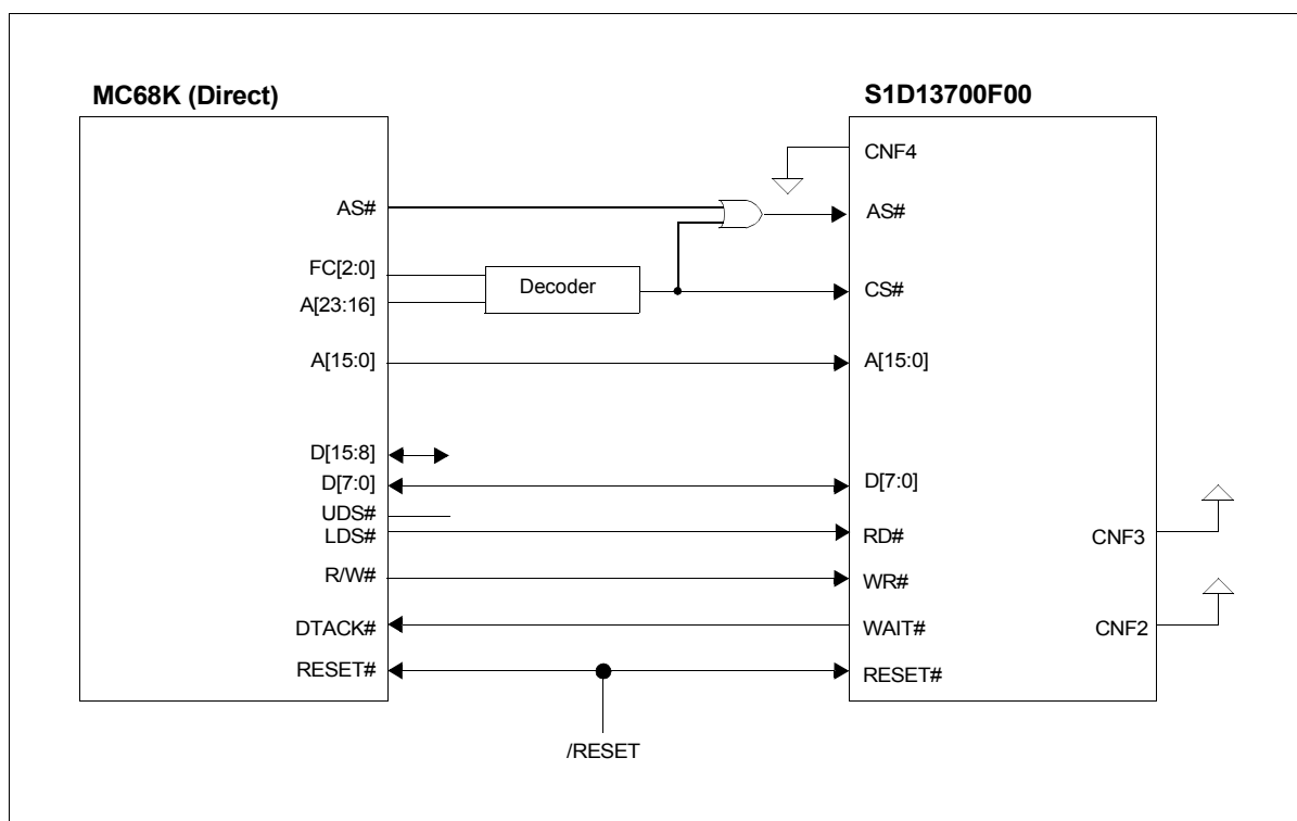
Figure 3-4 Direct MC68K to S1D13700F00 Interface Example
