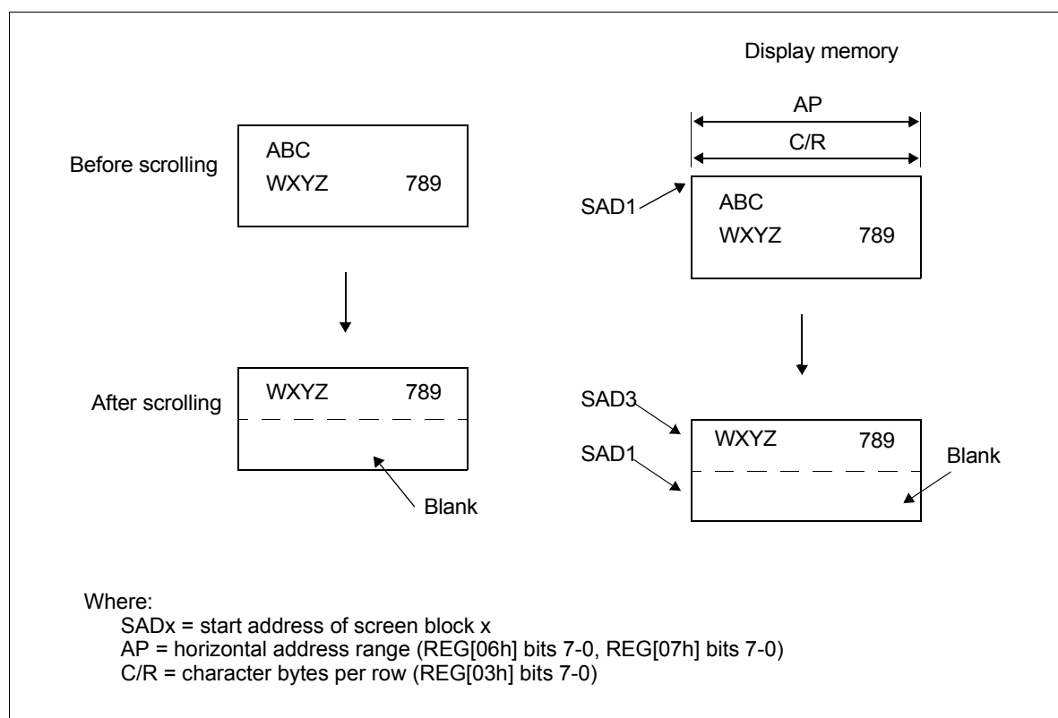
Figure 12-14 On-Page Scrolling
